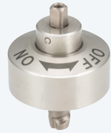
Knobless Heavy-Duty Quarter-Turn Clamps Clamping Force: 250, 400N
