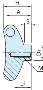
WN-N-SUS (Tapped)
