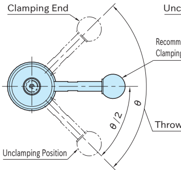
Counterclockwise Clamping
