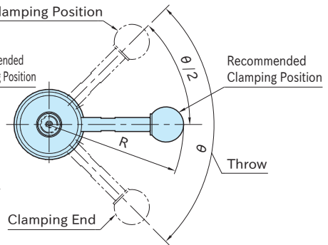
Clockwise Clamping
