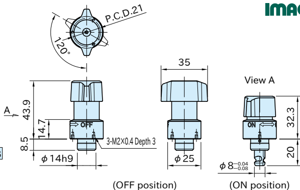
QCTHSA0825-20S (Metal Knob, ON position)
