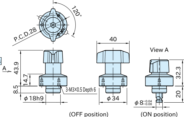
QCTHSA0834-20S (Metal Knob, ON position)
