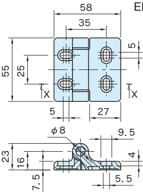
Section X-X
