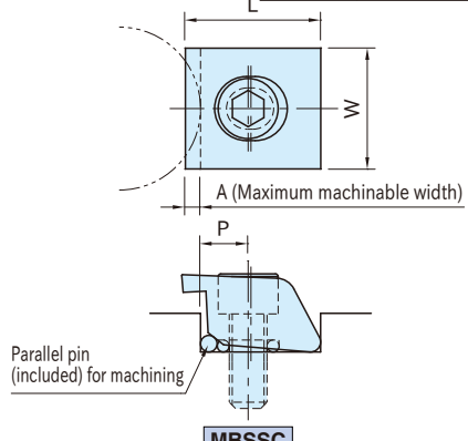
(Machinable edge)
