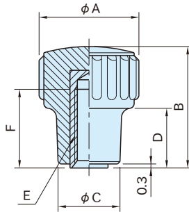
LKF (Tapped)
