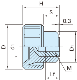
FTK FTK-SUS (Tapped Blind)
