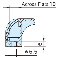
ESH-H Back Mounting
