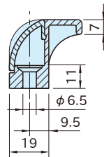
ESH-S Front Mounting
