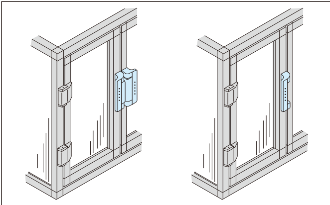
Mounting on single swinging or gatefold doors
