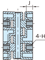
EMH-SS (Tapped)
