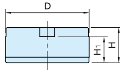
(Straight Type)
