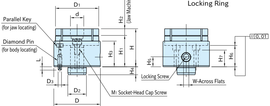
Locking Ring
