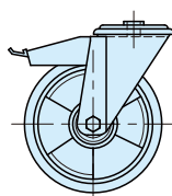
CAF5-FSF (Swivel Bracket with Through Hole & Brake)
