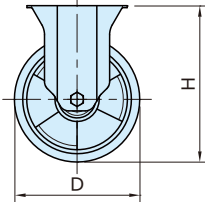
CAF5-PSL CAF5-PSL-H (Fixed Bracket)
