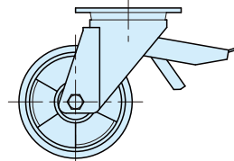
CAF5-150SSF-H CAF5-200SSF-H (Swivel Bracket with Brake)
