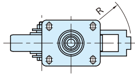
CAF5-PSL CAF5-PSL-H (Fixed Bracket)
