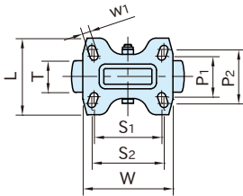
CAF5-PSL (Fixed Bracket)
