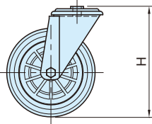
CAE2-FBL (Swivel Bracket with Through Hole)
