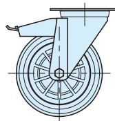
CAE2-SBF (Swivel Bracket with Brake)
