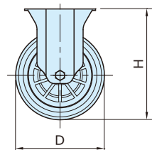
CAE2-PBL (Fixed Bracket)
