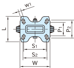
CAE2-PBL (Fixed Bracket)
