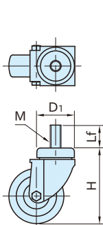
CAC7-CBL (Swivel Bracket with Stud)
