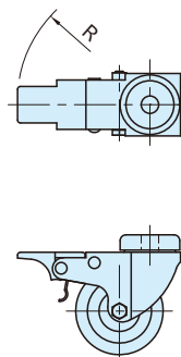
CAC7-FBF (Swivel Bracket with Through Hole & Brake)
