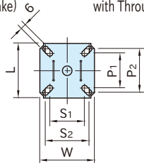
CAC7-FBL (Swivel Bracket with Through Hole)
