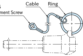
BLP-C1 (Cable)
