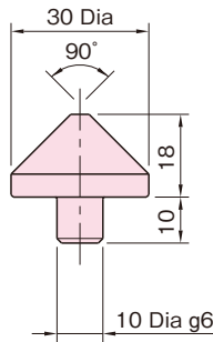
BJ733-10180 Conical Tip
