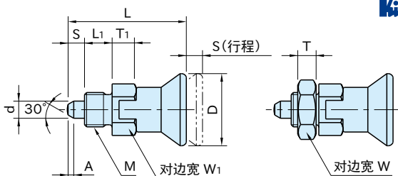
NDXNS-L NDXNS-AL-SUS (单螺母)
