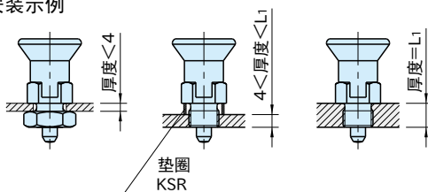
NDXNS-L NDXNS-AL-SUS (单螺母)
