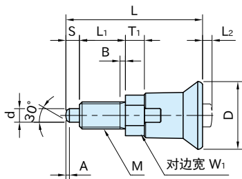
BNDXN BNDXN-A-SUS (单螺母)
